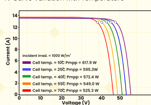
IV Curves for Front-Side Illumination of 595 Wp Panel
